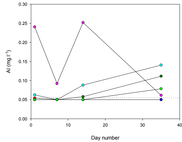
Figure 3-1 Contaminant and metalloid dynamics results for Paringa Paddock (12087) wetland soil materials for pH, SEC, Eh, silver (Ag), aluminium (Al) and arsenic (As).
