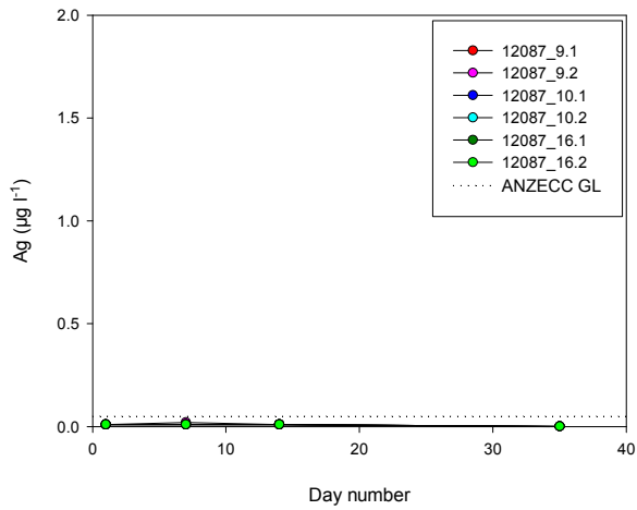
Figure 3-1 Contaminant and metalloid dynamics results for Paringa Paddock (12087) wetland soil materials for pH, SEC, Eh, silver (Ag), aluminium (Al) and arsenic (As).
