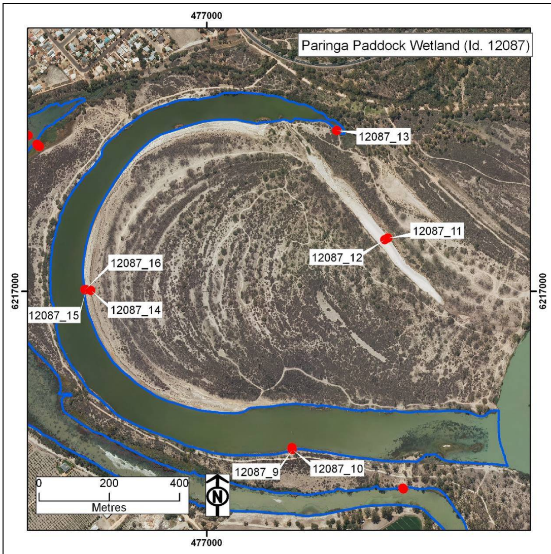
Figure 1-1 Paringa Paddock (12087) wetland aerial photograph with Phase 1 sampling sites identified.
