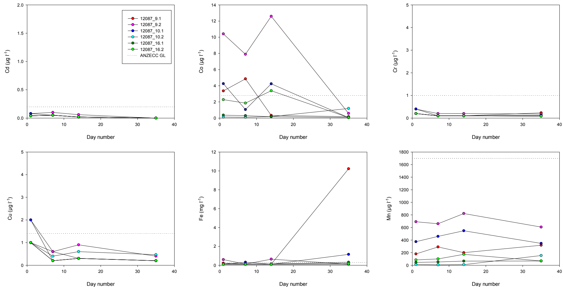
Figure 3-2 Contaminant and metalloid dynamics results for Paringa Paddock (12087) wetland soil materials for cadmium (Cd), cobalt (Co), chromium (Cr), copper (Cu), iron (Fe) and manganese (Mn).
