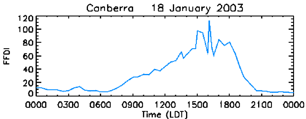
Figure 2. Time series of FFDI on 18 January 2003 at Canberra, ACT. Values are computed every 30 minutes from automatic weather station data.
