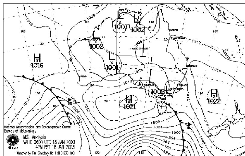
Figure 6. Mean sea level pressure analysis for 0600 UTC (5 pm Australian Eastern Daylight-savings Time) on 18 January 2003.
