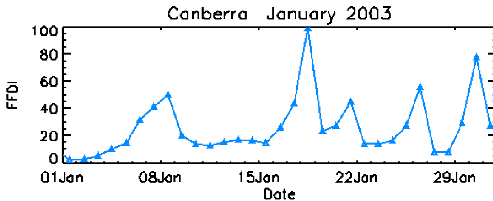
Figure 3. Time series of daily FFDI for Canberra, ACT during January 2003
