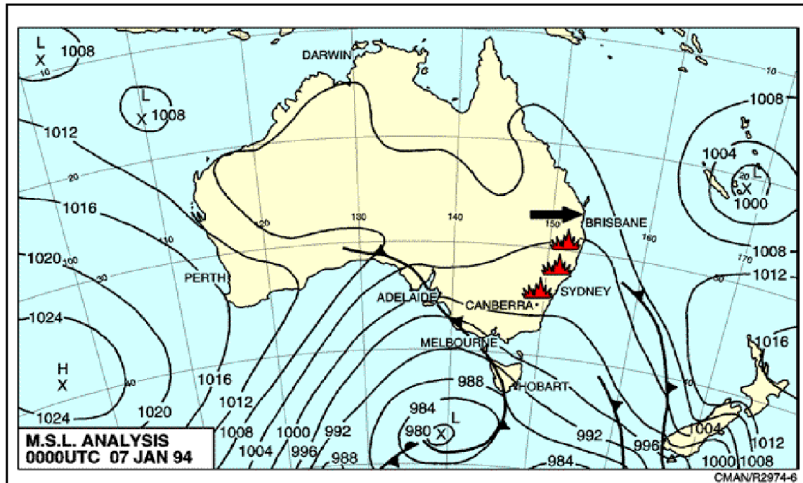
Figure 5. Mean sea level pressure contours (hPa) for 0000 UTC (11am Australian Eastern Daylight-savings Time) 7 January 1994.
