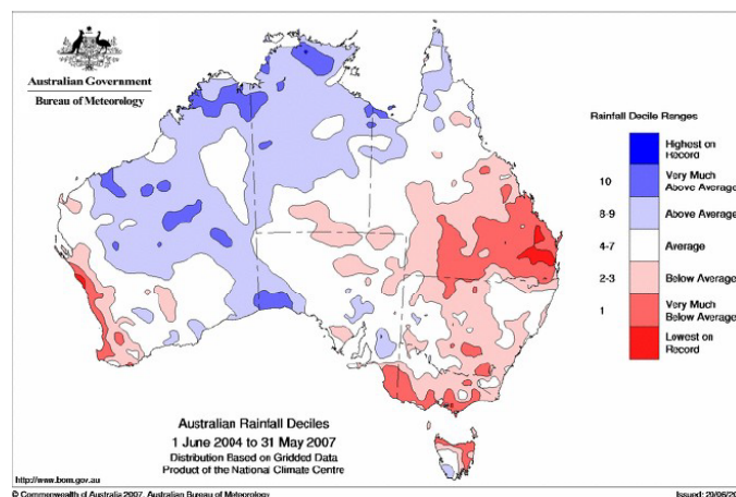
Figure 30. Rainfall deciles for Australia from June 2004 through May 2007. From http://www.bom.gov.au/cgi-bin/silo/rain_maps.cgi
