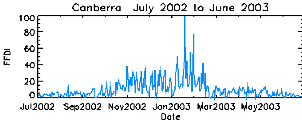
Figure 8. Time series of daily FFDI for Canberra, ACT, for the period from July 2002 through June 2003.
