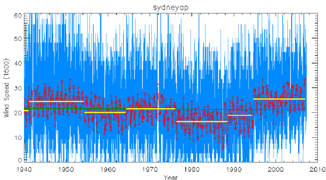
Fig. 13. Time series of 3 pm daily wind speed (blue; \text{km h}^{-1} ) at Sydney airport from 1940-2007. Red lines show monthly averages and horizontal yellow lines are the separate segments in a breakpoint (multi-phase regression) analysis.
