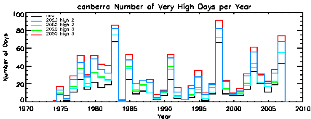
Figure 23. Time series showing changes in VHE fire danger days at Canberra for ‘now’ (1973-2006) and the equivalent days for the 2020 and 2050 ‘high’ scenarios in CCAM (Mark2) and CCAM (Mark3).
