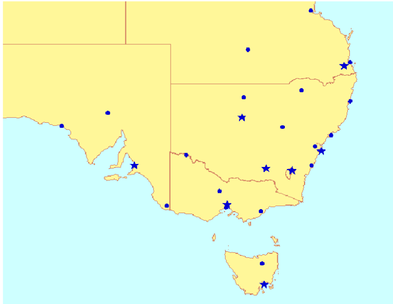
Figure 12. Map showing locations of stations used in this study. Circles represent stations with data extending to 1973. Stars represent stations where longer time series are available.
