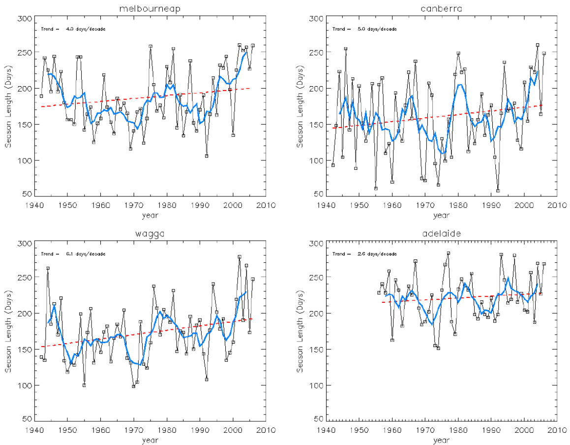
Figure 28. Estimated season length (days) at Melbourne AP, Canberra, Wagga and Adelaide calculated as described in the text. The blue line is the 5-year running mean. The red dashed line is the trend.
