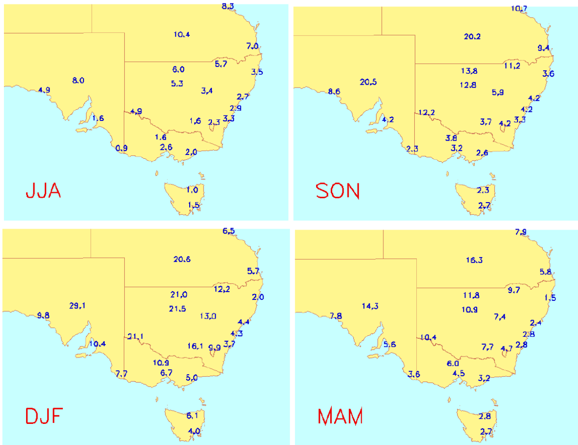
Figure 19. Map showing seasonal median FFDI values for 1973-2007. Seasons are notated in bottom left of each map. JJA = winter, SON = spring, DJF = summer and MAM = autumn.
