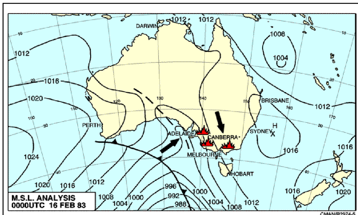
Figure 4. Mean sea level pressure contours (hPa) for 0000 UTC (11 am Australian Eastern Daylight-savings Time) 16 February 1983. Heavy arrows depict general wind direction and fire symbols denote approximate locations of bushfires observed on the day.
