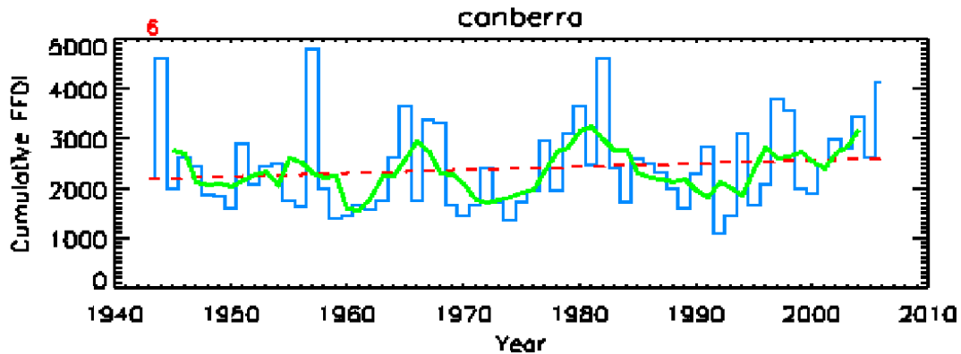
Figure 14. Annual \Sigma FFDI at Canberra from 1943-2007 (histogram). Also shown are the five-year running mean (green line) and the linear regression (red line). The trend (red number at top left) is +6 points per year.
