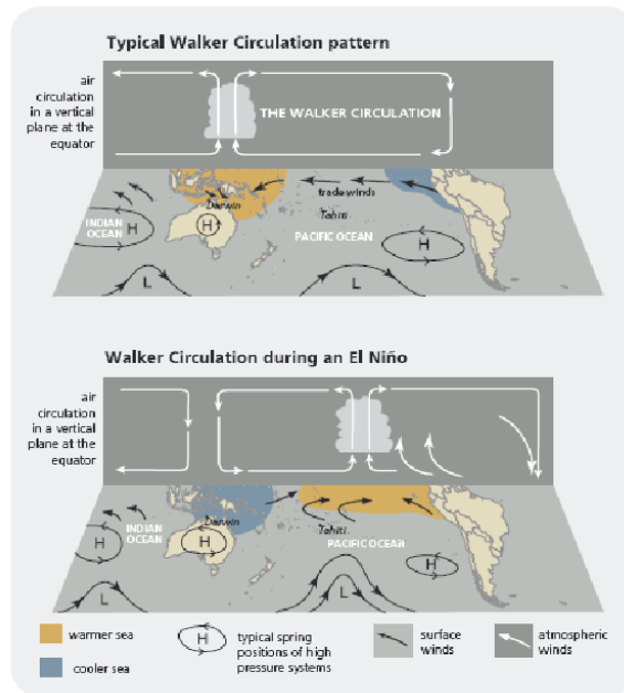
Figure 10. Schematic diagram summarizing the El Niño-Southern Oscillation phenomenon. Taken from http://www.bom.gov.au/info/leaflets/nino-nina.pdf .
