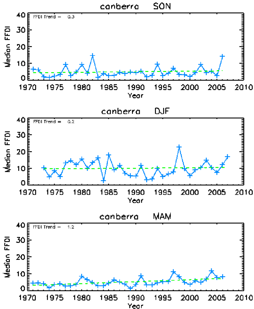
Figure 16. Seasonal median FFDI at Canberra for SON (spring, top), DJF (summer, centre) and MAM (autumn, bottom). Trend lines are shown in green. The value of the trend, in points per decade, is shown in the upper left corner of each plot.
