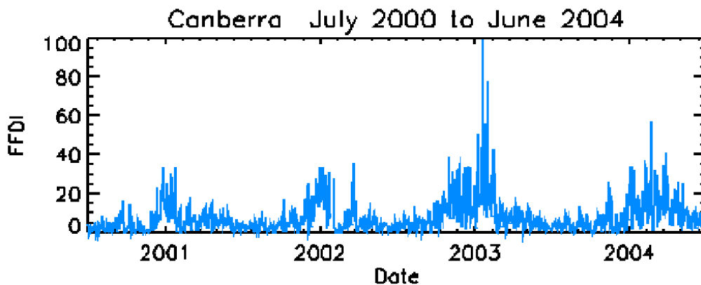
Figure 9. Time series of daily FFDI for Canberra, ACT, for the period from July 2000 through June 2004.
