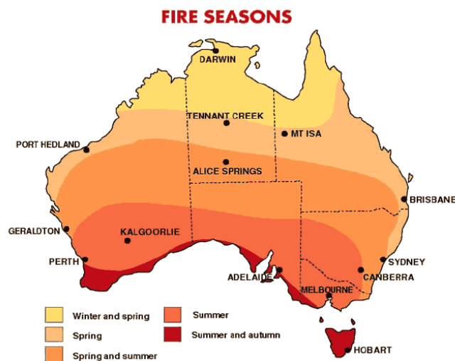
Figure 7. Map of peak fire seasons across Australia. From Luke and McArthur [1978].
