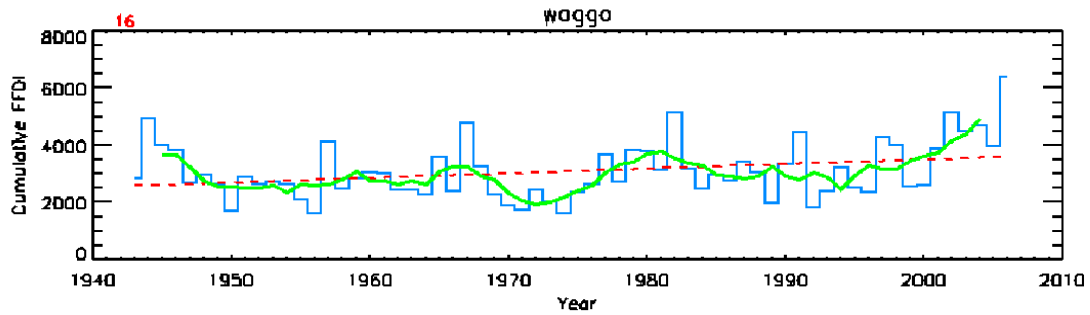
Figure 27. Time series of \Sigma FFDI at Wagga. The red line is based on linear regression and the red number at the top left indicates the trend. The green line is the 5-year running mean.
