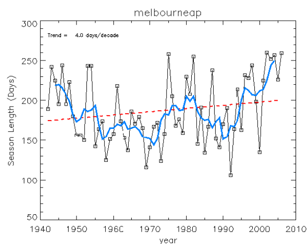
Figure E3: Estimated fire season length at Melbourne airport. The blue line is the 5-year running mean. The red dashed line is the line of best fit.
