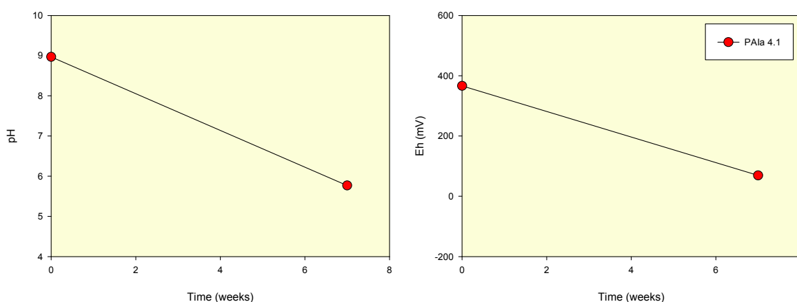
Figure 3-5 pH and Eh dynamics during monosulfide formation potential tests in surface soil sample PA1a4.1 from Paiwalla wetland.
