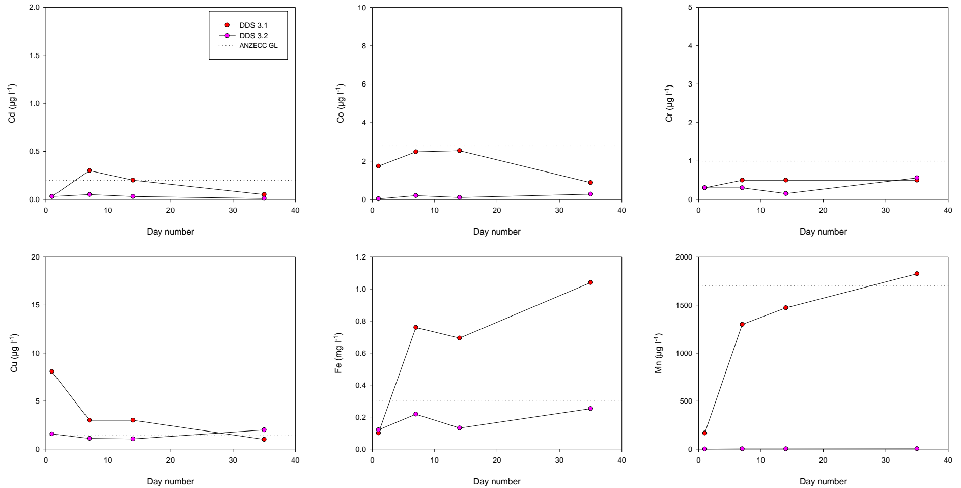
Figure 3-2 Contaminant and metalloid dynamics results for Devon Downs South wetland soil materials for cadmium (Cd), cobalt (Co), chromium (Cr), copper (Cu), iron (Fe) and manganese (Mn).
