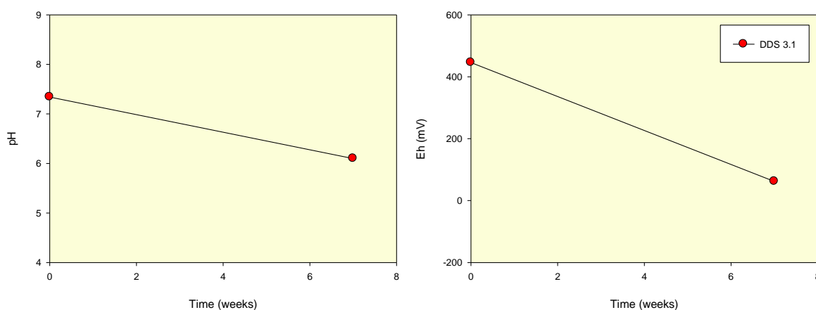
Figure 3-5 pH and Eh dynamics during monosulfide formation potential tests in surface soil sample DDS 3.1 from Devon Downs South wetland.
