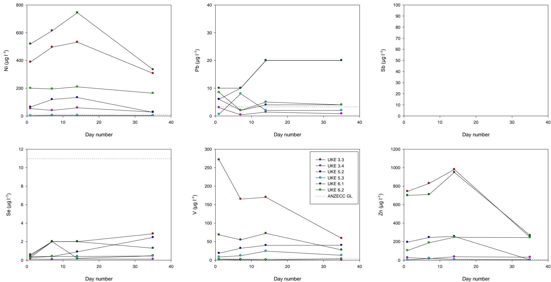
Figure 3-3 Contaminant and metalloid dynamics results for Ukee Boat Club wetland soil materials for nickel (Ni), lead (Pb), antimony (Sb), selenium (Se), vanadium (V) and zinc (Zn).
