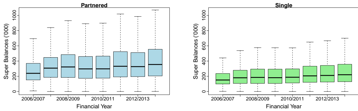
Figure 4.7: Box plots of superannuation balances at or up to one year after retirement, split by financial year of retirement. The right (green) plot shows single person households; the left (blue) plot shows couples where both partners retire in the same FY. All accounts within each household are combined.
